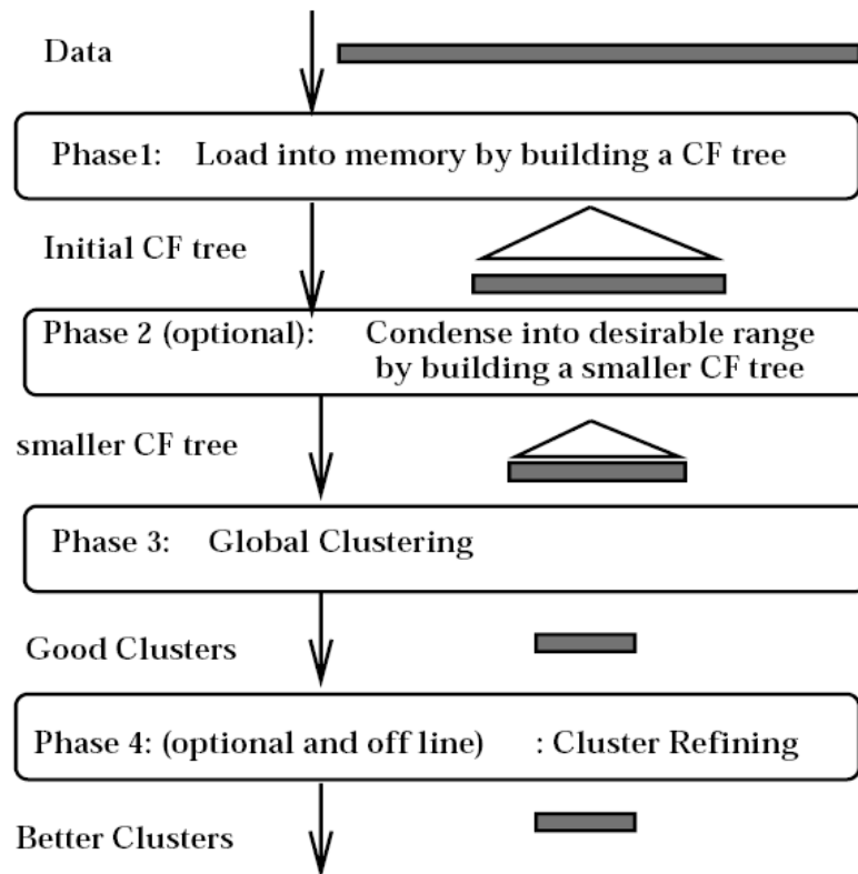
Figure: 13 Different phases of BIRCH algorithm
